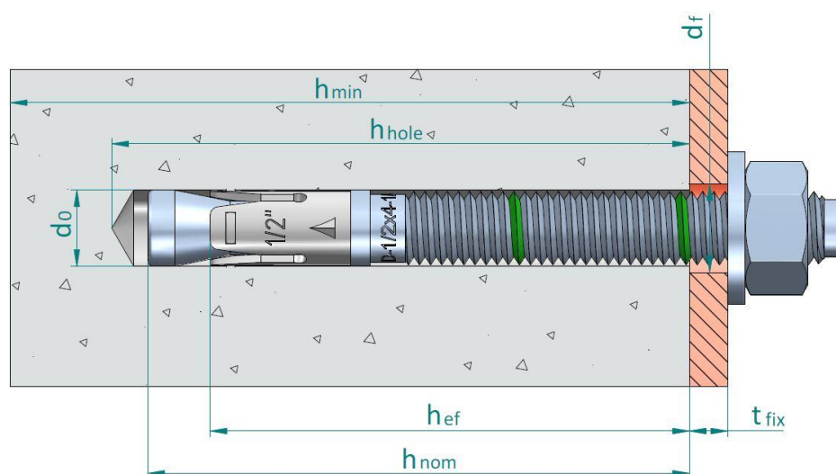
FIGURE 1—ANCHOR DIMENSIONS
