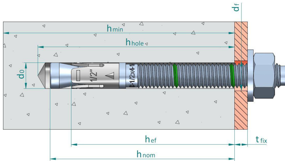
FIGURE 1—ANCHOR DIMENSIONS
