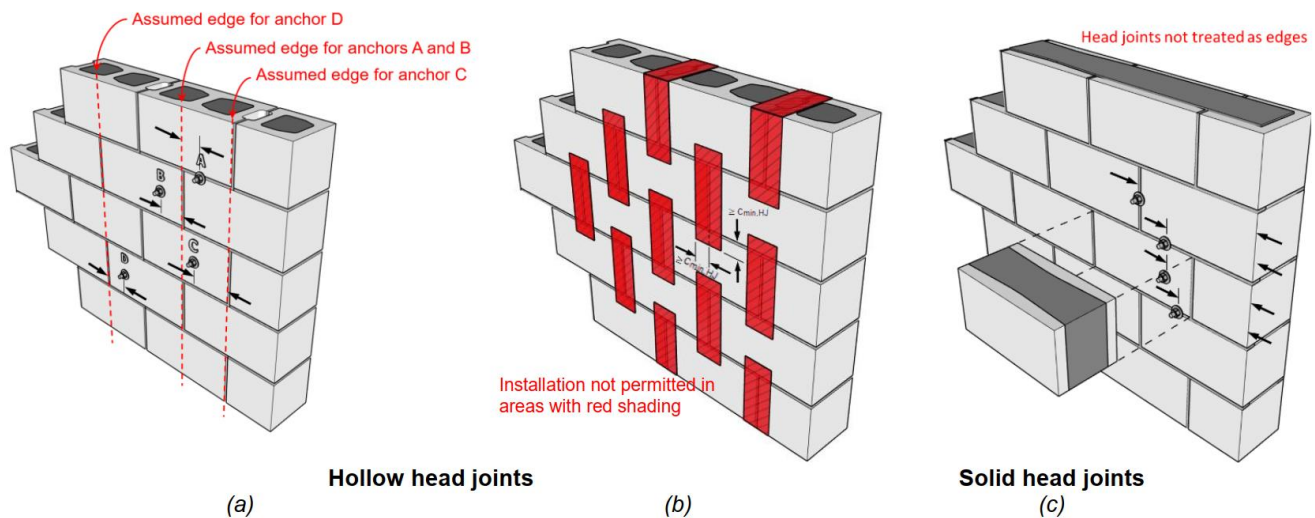
FIGURE 2—(a) Edge distance considerations in fully grouted CMU construction with hollow head joints, (b) exclusion zones in fully grouted construction with hollow head joints, and (c) edge distance considerations in fully grouted CMU construction with solid head joints. Note: dimensions to upper and lower edges omitted for clarity.
