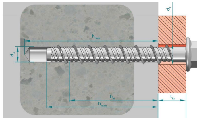
FIGURE 1—ANCHOR DIMENSIONS
